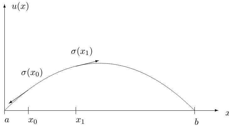
Figure 1.3: oscillating string
