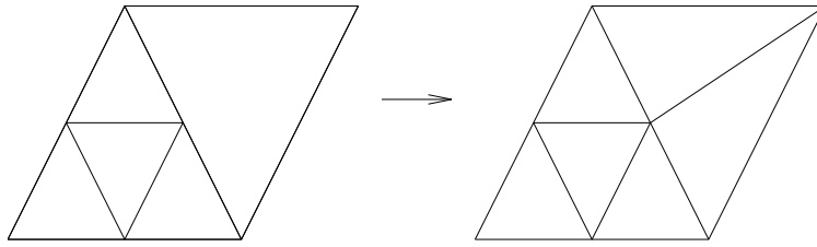
Figure 6.6: irregular closure
