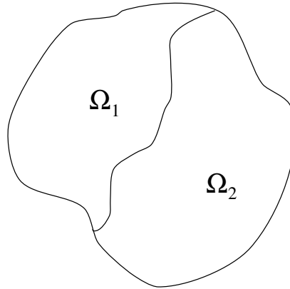
Figure 5.1: transition problem
