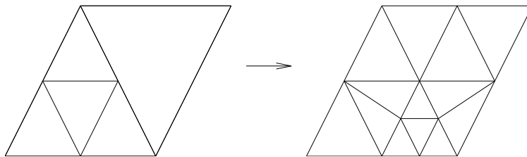
Figure 6.8: refinement without multiple irregular closures
