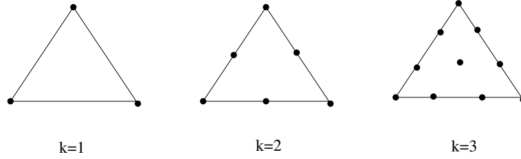
Figure 6.2: nodes
