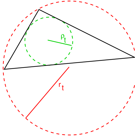
Figure 6.4: Incircle and circumcircle \rho_t and r_t of a triangle.
