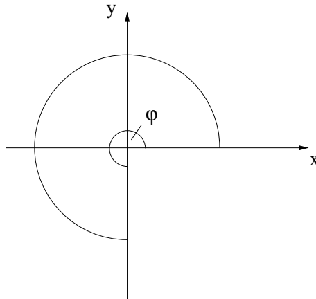
Figure 3.1: reentrant corner
