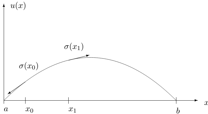
Figure 1.3: oscillating string
