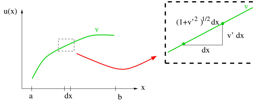
Figure 1.1: Calculation of the arc length l(a, b) of the graph of a function v = v(x) as l(a, b) = \int_a^b \sqrt{1 + v'(x)^2} dx . Here v' = v_x is the derivative of v . The two-dimensional generalization yields the above formula for surfaces after deformation.
