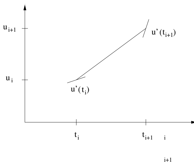
Figure 8.1: integration step
