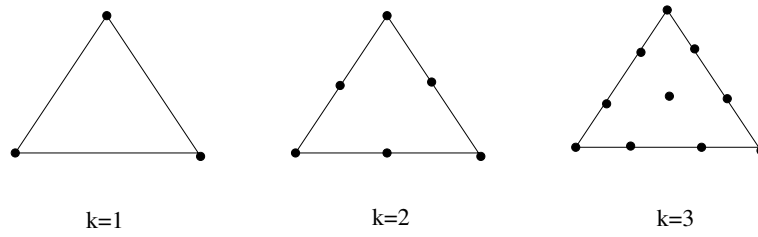
Figure 6.2: nodes
